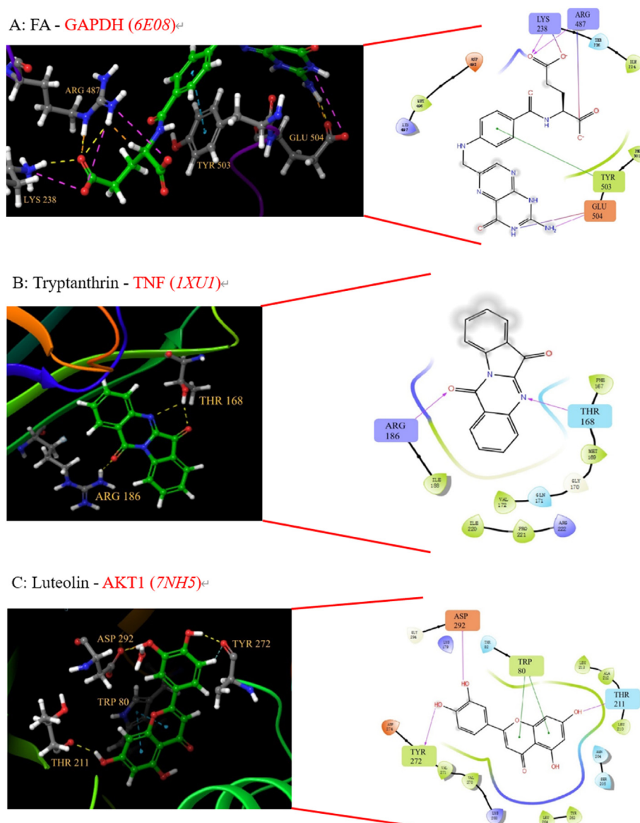
Fig. 2. The molecular docking modes of active compounds with target genes. (A) Action mode of FA with GAPDH (6E08); (B) Action mode of tryptanthrin with TNF (1XU1); (C) Action mode of luteolin with AKT1 (7NH5).
