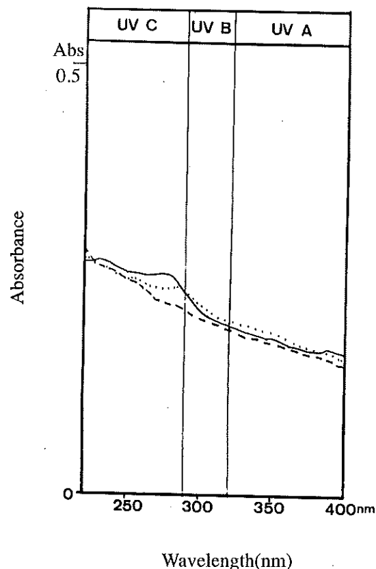
Figure 2. Absorption spectrum of Hypericum patulum (——), Hypericum pseudopetiolatum (.....), Hypericum sampsonii (-----).
