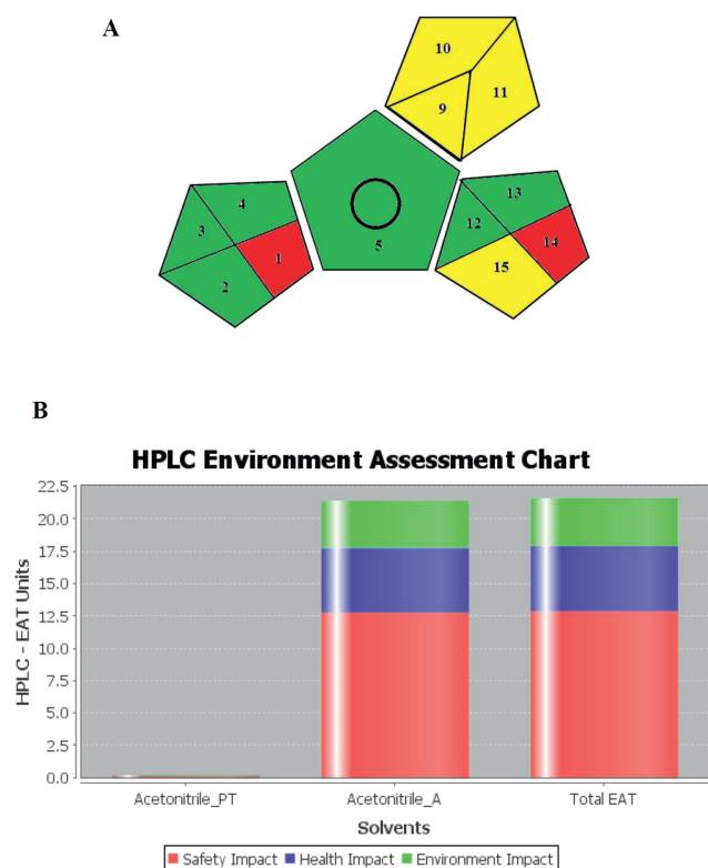
Fig. 4 – (A) GAPI pictogram for the developed HILIC method (references to numbers shown in the pictogram are provided in Supplementary Material Tables S1) and (B) HPLC-EAT chart for the developed HILIC method (Acetonitrile_PT: acetonitrile in the standard solution, Acetonitrile_A: acetonitrile in the mobile phase).
