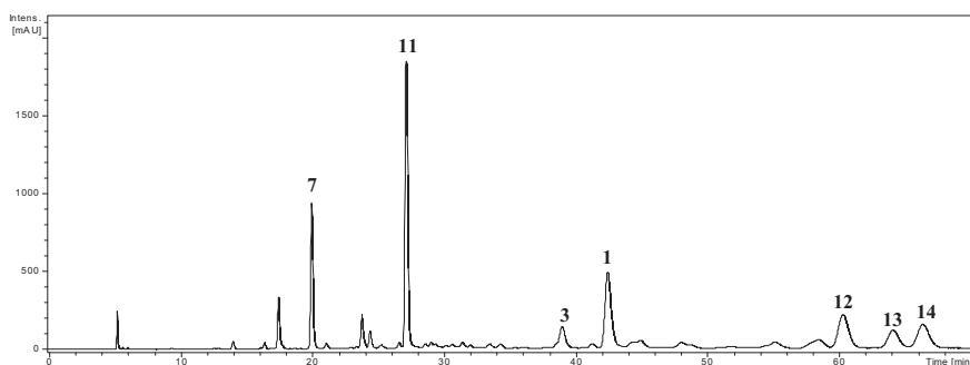
Fig. 3 – RP-18 HPLC chromatogram of fr. E4, detected at 280 nm, under an optimized condition as indicated in Section 2.4 for HPLC-SPE-NMR. Intens., intensity.
