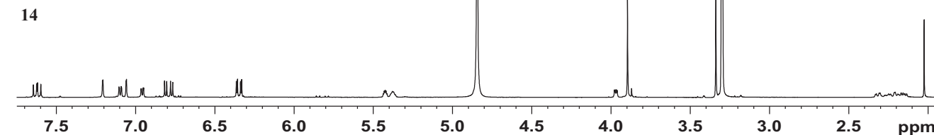
Fig. 4 – 1 H NMR spectra of compounds 1, 3, 7, and 11–14 (CD 3 OD), adopted from HPLC-SPE-TT-NMR of fr. E4.
