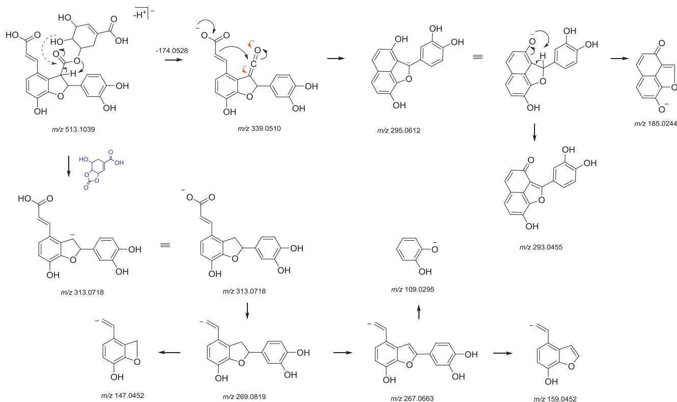
Fig. 3 – Putative fragmentation pathway of compound 12 . Measured exact mass of each fragment ion, as listed in Table 1, was at m/z within 5 ppm vs. its relative theoretical m/z value. This latter is reported below each structure.
