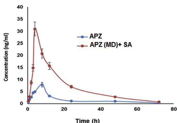
Fig. 3 – Mean plasma concentration time profiles of APZ (3 mg/kg) and APZ with SA (20 mg/kg) dose in rats for 15 days daily. Each value is expressed as mean \pm SD (n = 6).
