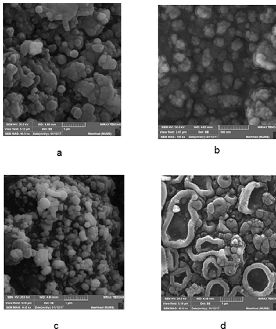
Fig. 2 – SEM images of: (a) MIP-PPY-PGE, (b) AgNPs-MIP-PGE before template extraction (c) AgNPs-NIP-PGE and (d) AgNPs-MIP-PPY after template extraction.
