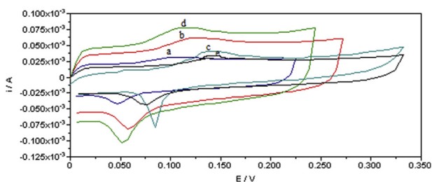
Fig. 4 – Cyclic voltammograms of different electrodes in 10 mM K 3 Fe(CN) 6 . (a) Unremoved MEB-MIP-GPE, (b) Bare GPE, (c) Unremoved MEB-AgNPs-MIP-GPE, (d) Removed MEB AgNPs-MIP-GPE and (e) After incubation of AgNPs-MIP-PGE in MEB solution.
