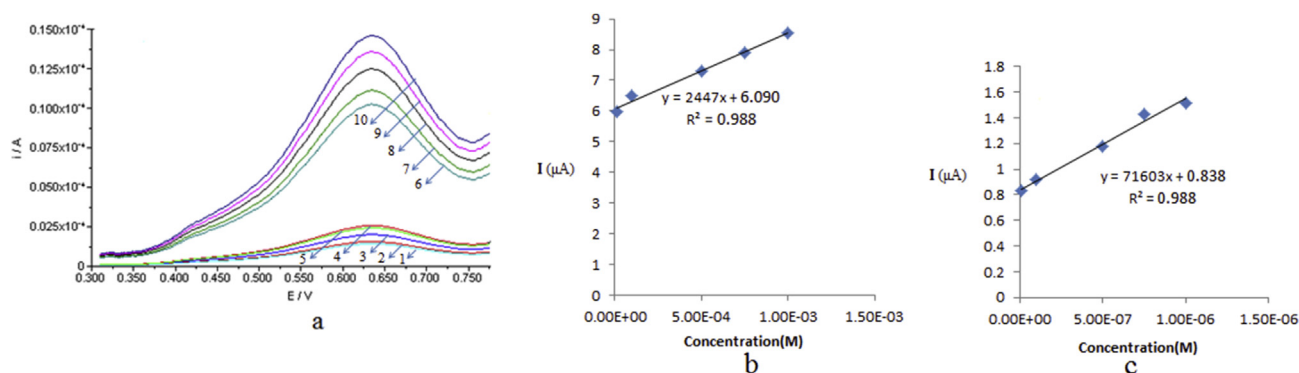
Fig. 8 – (a) The differential pulse voltammograms for different concentrations of MEB using AgNPs-MIP-PGE in BRB pH 6.5, at a scan rate of 16 \text{mV s}^{-1} . The voltammograms are: 1, 2, 3, 4, 5, 6, 7, 8, 9 and 10 are related to the MEB concentrations at 1 \times 10^{-8} M, 1 \times 10^{-7} M, 5 \times 10^{-7} M, 7.5 \times 10^{-7} M, 1 \times 10^{-6} M, 1 \times 10^{-5} M, 1 \times 10^{-4} M, 5 \times 10^{-4} M, 7.5 \times 10^{-4} M and 1 \times 10^{-3} M, respectively. (b) and (c) The calibration curve of the peak current values against the concentration of MEB.
