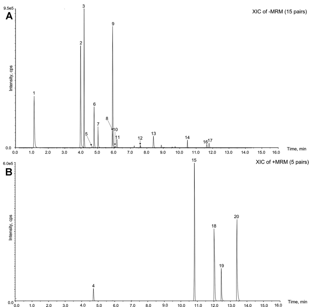
Fig. 1 – The XICs of the 20 analytes in sample 4 by UHPLC–MS/MS, 15 pairs in negative ion (A) and 5 pairs in positive method (B), respectively.
