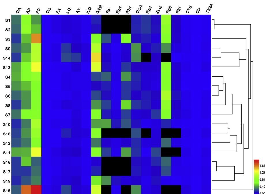
Fig. 3 – Dendrogram and heatmap of HCA of 19 WJBFP samples, S1–S19 represent 19 batches of WJBFP. Red color corresponds to higher concentration, while blue color corresponds to lower concentration. And the black color represents trace concentration.
