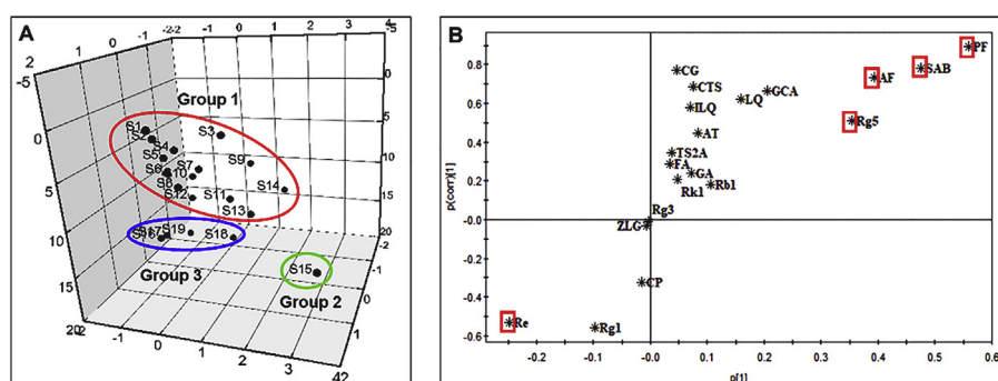
Fig. 2 – Scores (A) and loadings (B) plots of PCA. (A) refer to the sample number, S1–S19 represent 19 batches of WJBFP. The 20 compounds are shown in (B).
