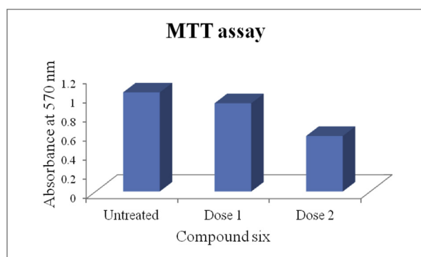
Fig. 3 – MTT assay. MTT assay revealed effectiveness of compound six at two different doses with higher cytotoxicity at dose 2 than dose 1. Dose 1 is 20 µg/ml and dose 2 is 80 µg/ml.
