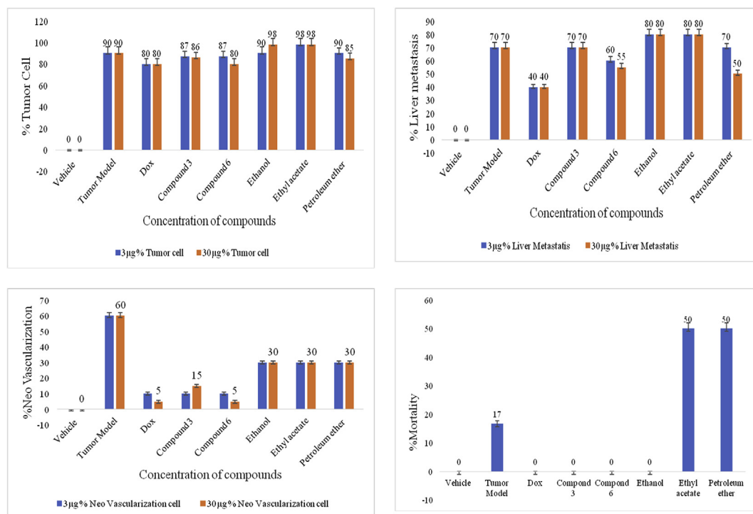
Fig. 5 – In vivo cytotoxicity evaluation of bioactive compounds. (A) Percentage tumor cell after treatment with samples. The ethyl iso-allocholate at the dose of 30 \mu\text{g} showed maximum growth inhibitory effect, equivalent to doxorubicin (positive control) i.e. 80 \pm 5 . (B) Percentage liver metastasis. The ethyl iso-allocholate and petroleum ether fraction showed least percentage liver metastasis i.e. 55 \pm 3 and 50 \pm 3 , respectively. (C) Percentage neo-vascularization. The ethyl iso-allocholate treated group showed significantly less formation of new blood vessels ( **P < 0.01 ) i.e. 5 \pm 0.8 as compared to the negative control group which was 60 \pm 2 . (D) All the compounds showed zero percent mortality except ethyl acetate and petroleum ether fraction. dox refers to doxorubicin, compound 3 is benzenepropanoic acid, 3,5-bis (1,1-dimethylethyl)-4-hydroxy, methyl ester and compound 6 is ethyl iso-allocholate.
