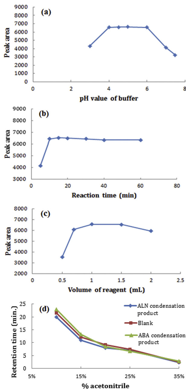
Fig. 1 – Effect of (a) the buffer pH values, (b) the reaction time and (c) the volume of reagent on the peak area of ALN condensation product obtained from the reaction of 500 µg mL -1 ALN with the pre-column derivatizing reagent and (d) effect of % acetonitrile in mobile phase on the retention times of ALN condensation product, ABA condensation product and blank obtained from the reaction of 500 µg mL -1 ALN and 2.5 µg mL -1 ABA with the pre-column derivatizing reagent.
