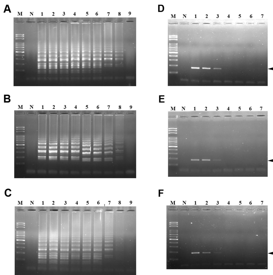
Fig. 2 – The sensitivity of specific LAMP and PCR primers used for the detection of EBN. Three kinds of EBN samples, white EBN (A), yellow EBN (B) and red EBN (C), were prepared for LAMP assay. Lanes M and N represent the 100 bp DNA ladder and the negative control, respectively. Lanes 1–9 represent the different amounts of EBN DNA added to the LAMP reaction: 1, 10^{-1} \mu g; 2, 10^{-2} \mu g; 3, 10^{-3} \mu g; 4, 10^{-4} \mu g; 5, 10^{-5} \mu g; 6, 10^{-6} \mu g; 7, 10^{-7} \mu g; 8, 10^{-8} \mu g; and 9, 10^{-9} \mu g. As to PCR primers used for the detection of EBN, also three kinds of EBN samples, white EBN (D), yellow EBN (E) and red EBN (F), were prepared for PCR assay. Lanes M and N represent the 100 bp DNA ladder and the negative control, respectively. Lanes 1–7 represent the different amounts of EBN DNA added to the reaction: 1, 10^{-1} \mu g; 2, 10^{-2} \mu g; 3, 10^{-3} \mu g; 4, 10^{-4} \mu g; 5, 10^{-5} \mu g; 6, 10^{-6} \mu g; 7, 10^{-7} \mu g. The black arrow represents the specific amplified PCR product in the agarose gel. Total 13 discrete DNA fragments contained in the 100 bp DNA Ladder s ranging in size from 3000, 2000, 1500, 1000, 900, 800, 700, 600, 500, 400, 300, 200 to 100 bp, sequentially.
