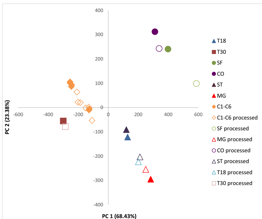
Fig. 4 – PC scores of fat or oil samples before and after yogurt production. C1– C6 corresponds to different milk fat samples, CO: Corn oil, MG: Margarine, SF: Sunflower oil, ST, T18, T30: Commercial vegetable fat blends.
