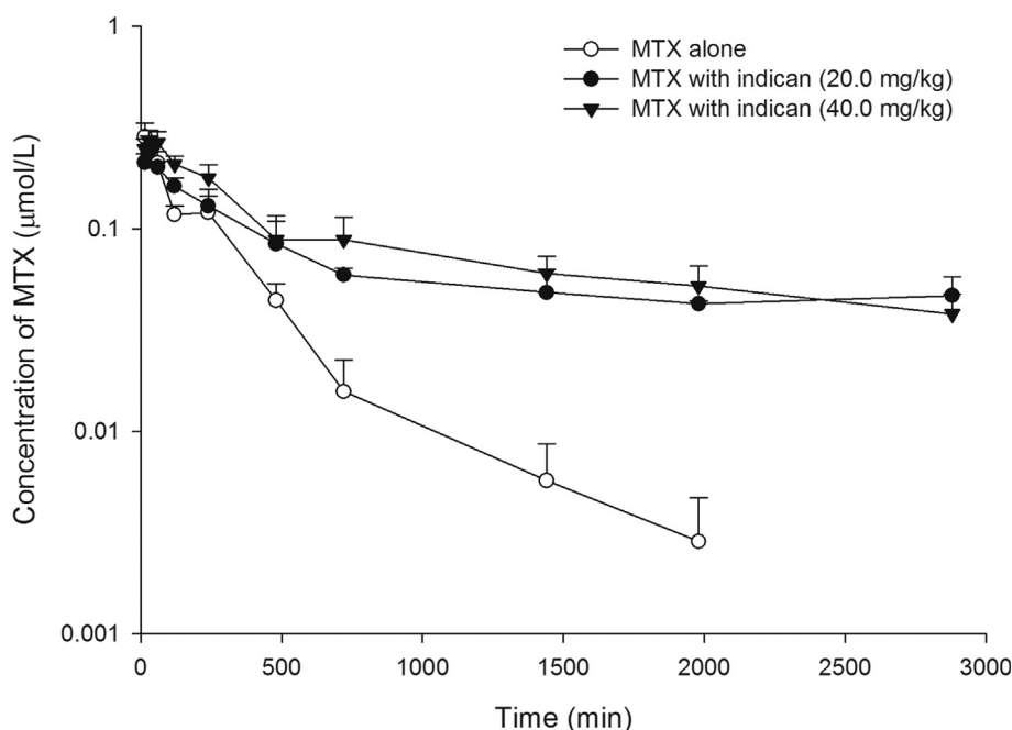
Fig. 2 – Mean ( \pm S.E.) serum semi-log concentration–time profiles of methotrexate (MTX) after oral MTX alone (5.0 mg/kg) ( \circ ), and coadministrations with 20.0 ( \bullet ) and 40.0 mg/kg ( \blacktriangledown ) of indican, revealing that the elimination of MTX was inhibited by both dosages of indican.
