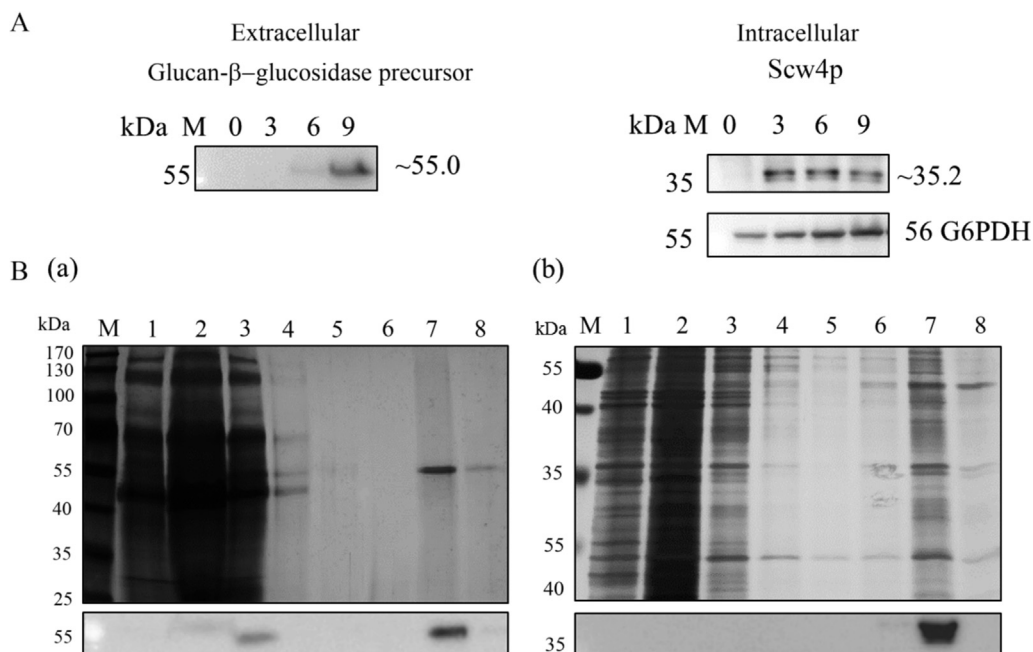
Figure 3 – Molecular cloning and purification of the glucan-β-glucosidase precursor and Scw4p. (A) Western blot analysis of the extracellular glucan-β-glucosidase precursor and intracellular Scw4p expressions in yeast transformants after 0 hour, 3 hours, 6 hours, and 9 hours of induction with galactose. (B) Purification of recombinant proteins with His tags by nickel columns. (a and b) The extracellular glucan-β-glucosidase precursor purification and the intracellular Scw4p purification, respectively. Each fraction collected from protein purification was analyzed by sodium dodecyl sulfate-polyacrylamide gel electrophoresis (SDS-PAGE) with silver staining (above) and Western blotting (bottom) using an anti-His antibody. Lane 1, flow through fraction; lanes 2–5, wash-step fractions; lanes 6–8, elution fractions from the protein purification process.
