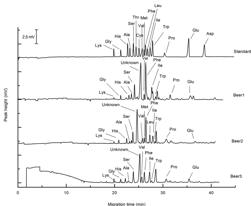
Figure 6 – Electropherograms of the three beer samples under optimized conditions. The conditions were as in Figure 4.
