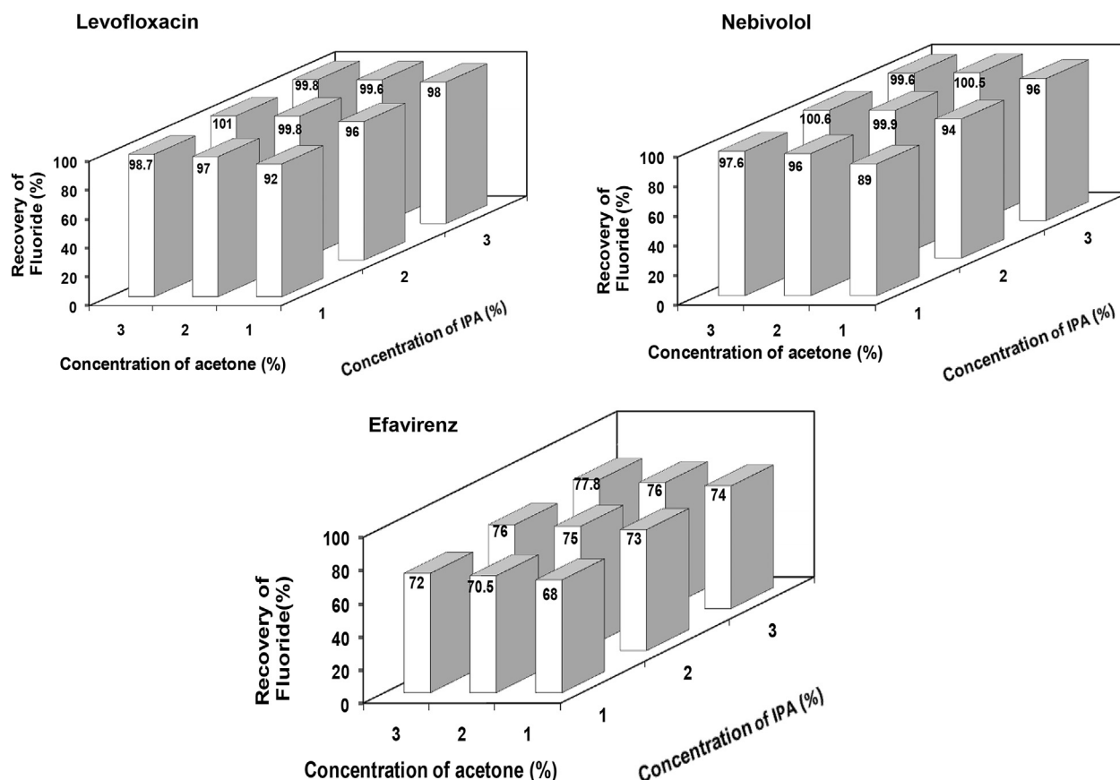
Figure 1 – Optimization of reagent composition (acetone and isopropyl alcohol) for the quantitative recovery of fluoride from the three representative samples; levofloxacin, nebulivol, and efavirenz; sample mass = 3 mg, volume of the reagent solution = 10 mL, UV irradiation time = 5 minutes.
