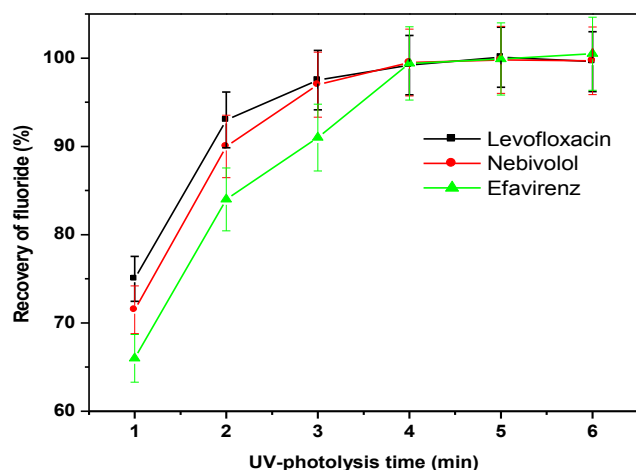
Figure 3 – Influence of UV irradiation time on the recovery of fluoride from the three representative samples (levofloxacin, nebivolol, and efavirenz). Sample mass = 3 mg, volume of the reagent solution = 10 mL, composition of reagent solution = 2% acetone + 2% IPA + 0.003% \text{Na}_2\text{CO}_3 .
