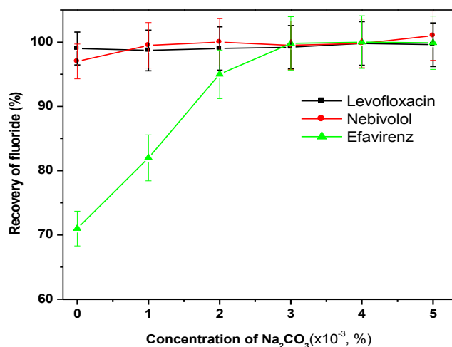
Figure 2 – Effect of concentration of \text{Na}_2\text{CO}_3 on the recovery of fluoride from the three representative samples (levofloxacin, nebulivol, and efavirenz) selected for UV-assisted decomposition studies. Sample mass = 3 mg, volume of the reagent solution = 10 mL, composition of reagent solution = 2% acetone + 2% IPA, UV irradiation time = 5 minutes.
