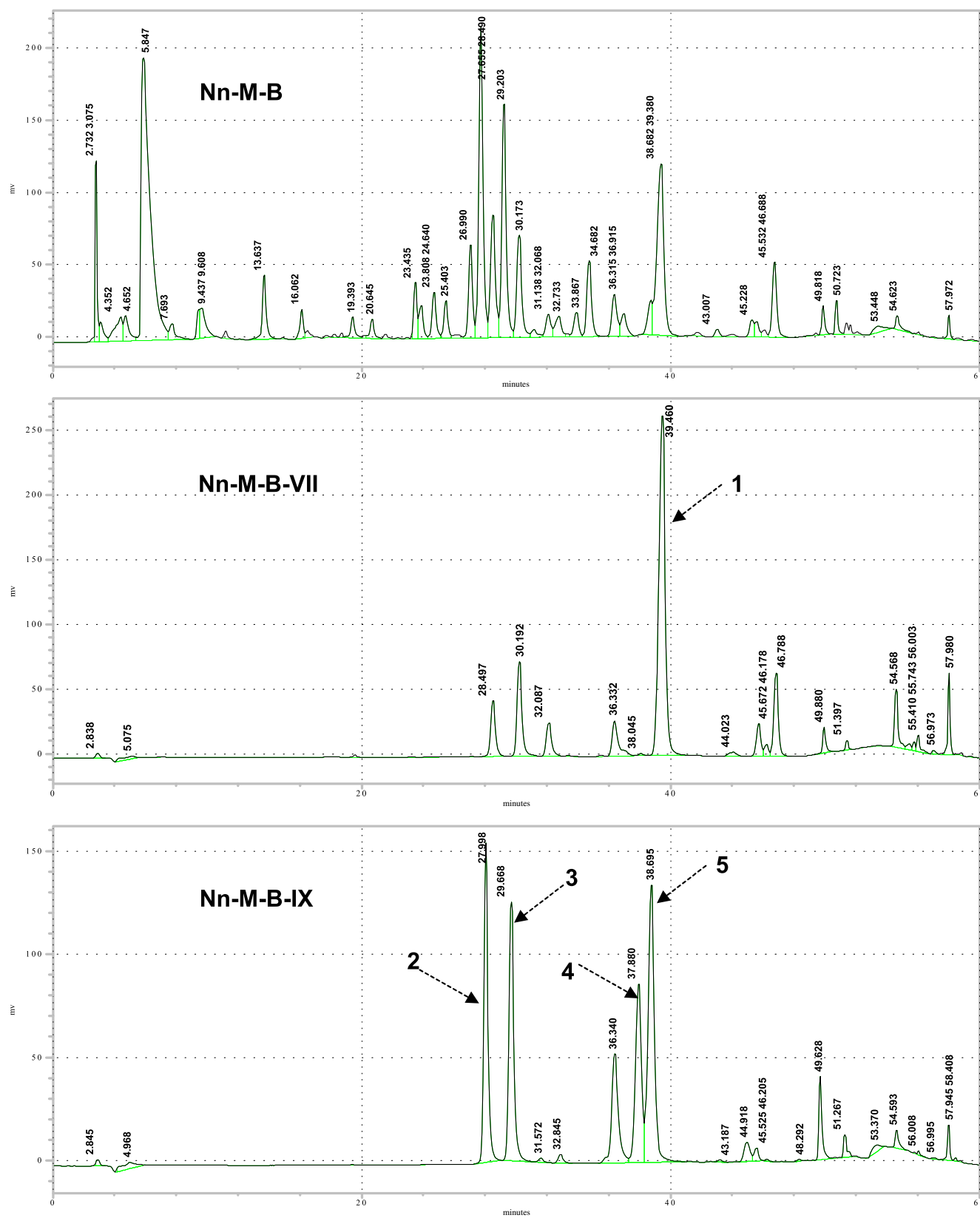
Figure 3 – Typical HPLC profile of the most active fractions of Nelumbo nucifera seed embryo. Rutin (1), orientin (2), isoorientin (3), isoquercitrin (4), and hyperoside (5) were detected at 254 nm. HPLC = high-performance liquid chromatography.
