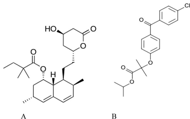
Figure 1 – Structures of (A) simvastatin and (B) fenofibrate.
