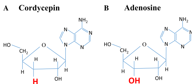
Figure 1 – The difference in the chemical structures of bioactive compounds, (A) cordycepin and (B) adenosine [6].
