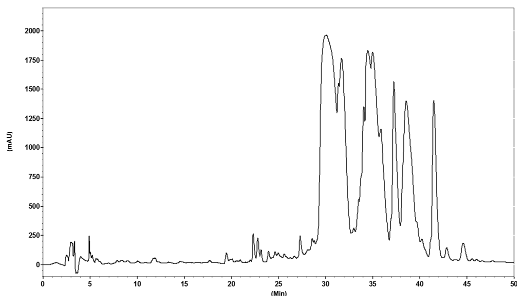
Figure 1 – Purification of camel milk protein hydrolysate on a C_8 semipreparative column ( 10 \times 250 \text{ mm}^2 ). The eluted fractions were numbered as indicated on HPLC chromatogram. Fractions named 1, 2, and 3 were further characterized. HPLC = high-performance liquid chromatography.
