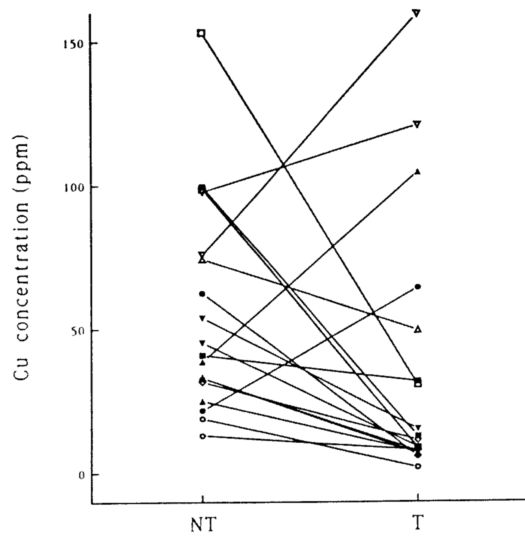
Figure 4. Copper concentrations in non-tumor (NT) and tumor (T) regions. Values were presented for each individual and the results were expressed as ppm. The means in NT and T regions were 56.5 and 36.2, respectively. P-value by Student's t-test was 0.12.
