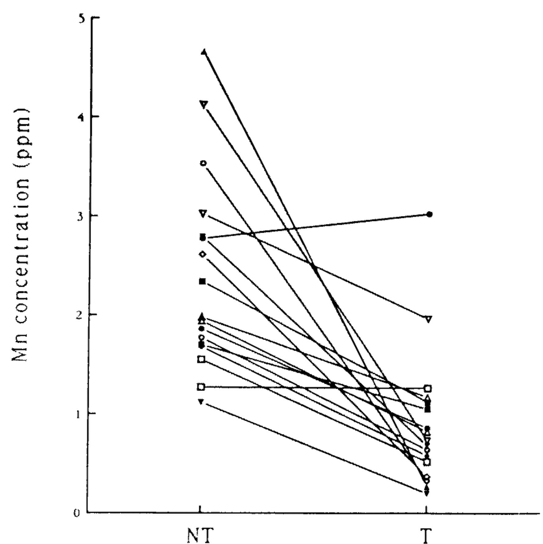
Figure 2. Manganese concentrations in non-tumor (NT) and tumor (T) Regions.
