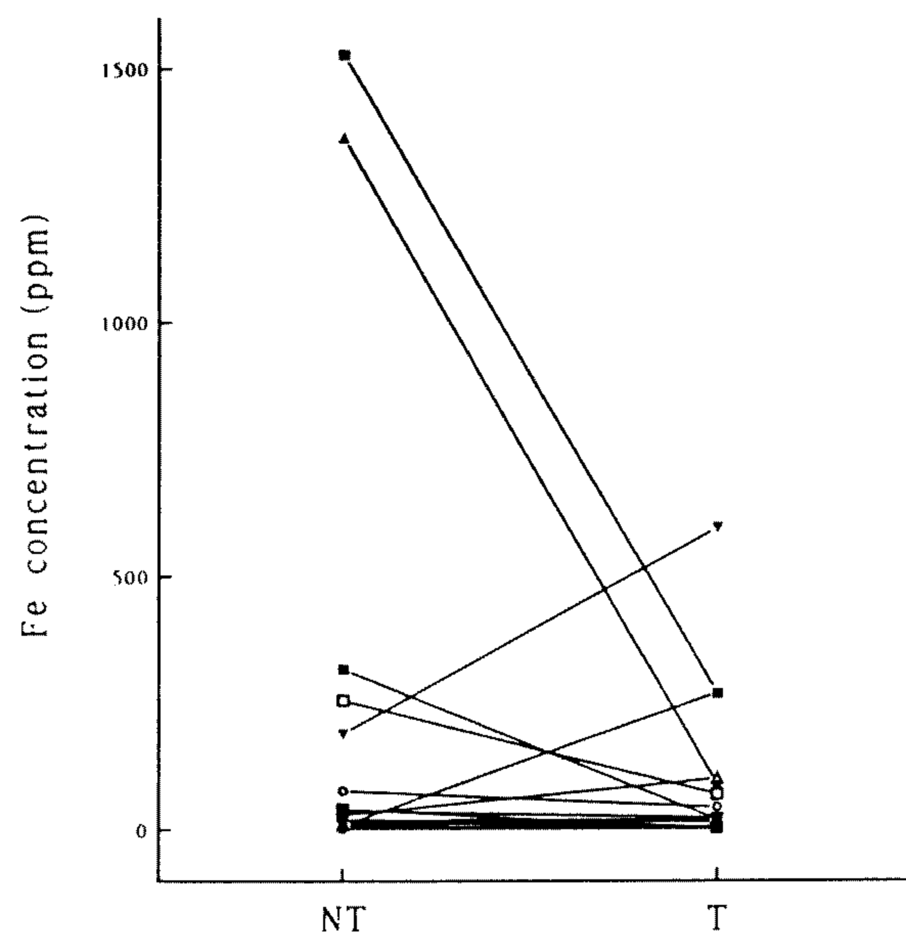
Figure 3. Iron concentrations in non-tumor (NT) and tumor (T) regions. Values were presented for each individual and the results were expressed as ppm. The means in NT and T regions were 66.2 and 77.4, respectively. P-value by Student's t-test was 0.78.
