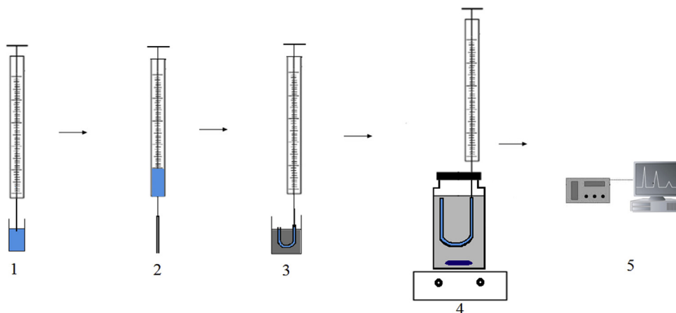
Fig. 1 – Different steps of hollow fiber liquid phase microextraction: (1) filling the syringe with acceptor phase; (2) filling the hollow fiber lumen with acceptor phase; (3) bending the hollow fiber into the U shape and its insertion into the aqueous sample; (4) agitation with stirring; and (5) instrumental analysis.
