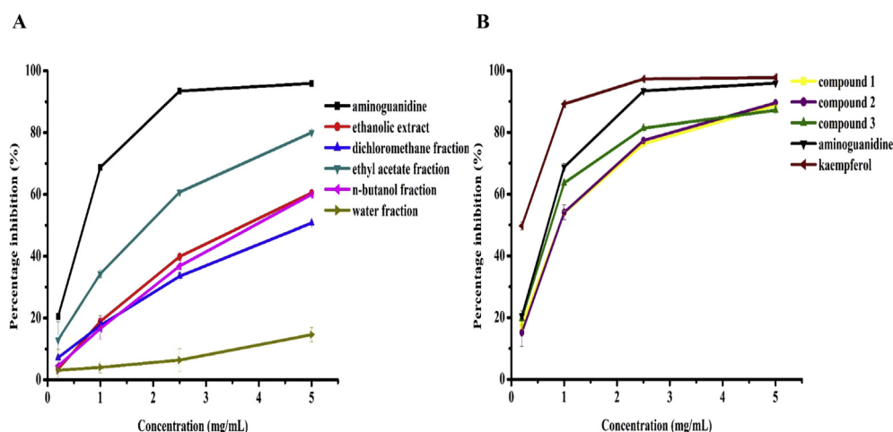
Fig. 3 – Effects on the AGE formation in BSA-methylglyoxal assay of aminoguanidine, the five fractions of CNC flowers (A) and the three compounds isolated from CNC flowers, kaempferol (B). Each value was expressed as mean \pm SD ( n = 3 ).
