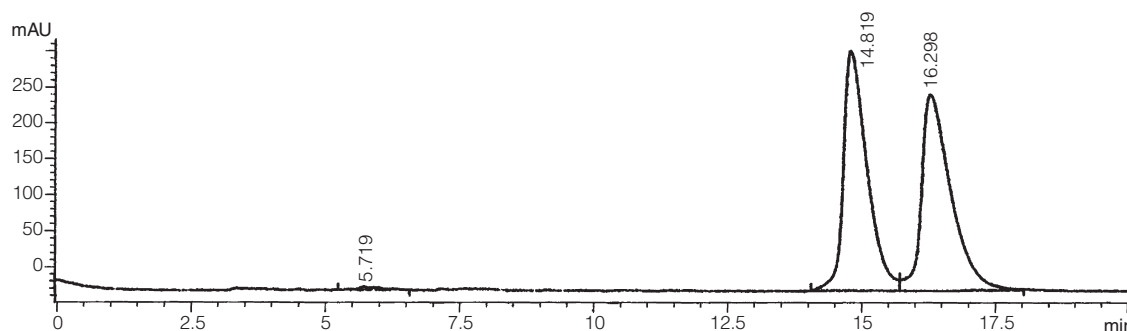
Figure 1. HPLC chromatogram of 1000 mg/L bifenthrin standard solution separated by Sumichiral OA-2500-I column. The mobile phase is n -hexane/isopropanol/methanol (99.8/0.06/0.14). The retention times of (-)-bifenthrin and (+)-bifenthrin are 14.819 min and 16.298 min, respectively.
