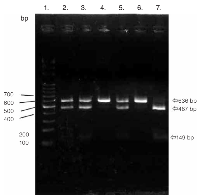
Figure 1. RFLP from the PCR products of Astragali Radix. Lane 1: 100 bp ladder marker, Lane 2: hybrid (AR-1), Lane 3: hybrid (Am31-5), Lane 4: A. membranaceus (Am31-6-2), Lane 5: hybrid (Am31-7), Lane 6: A. membranaceus (Am31-17), Lane 7: A. membranaceus var. mongholicus (Am31-24).
