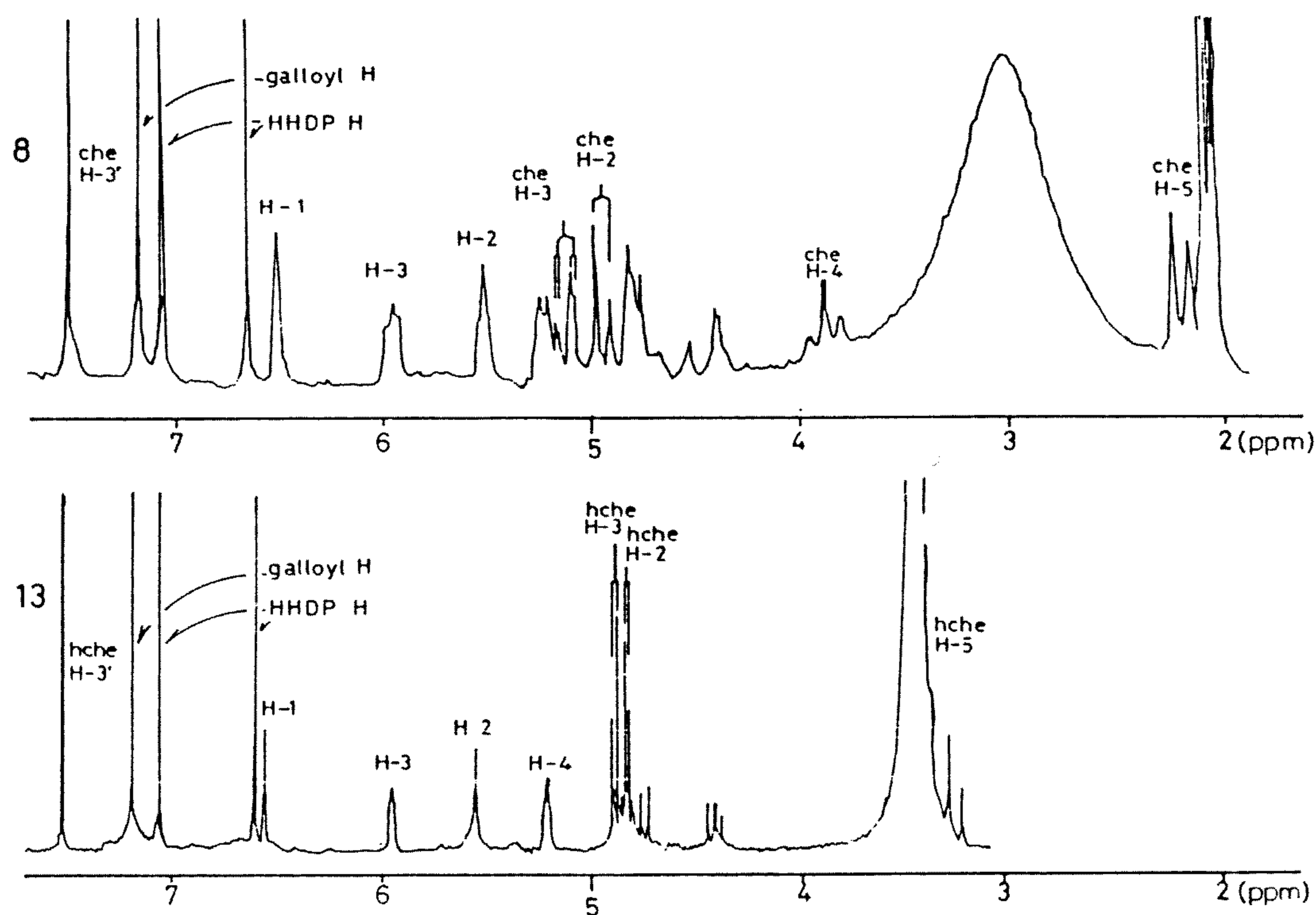
Figure 6. ^1\text{H-NMR} Spectra of Compounds 8 (100 MHz) and 13 (270 MHz) (in acetone- \text{d}_6 )
