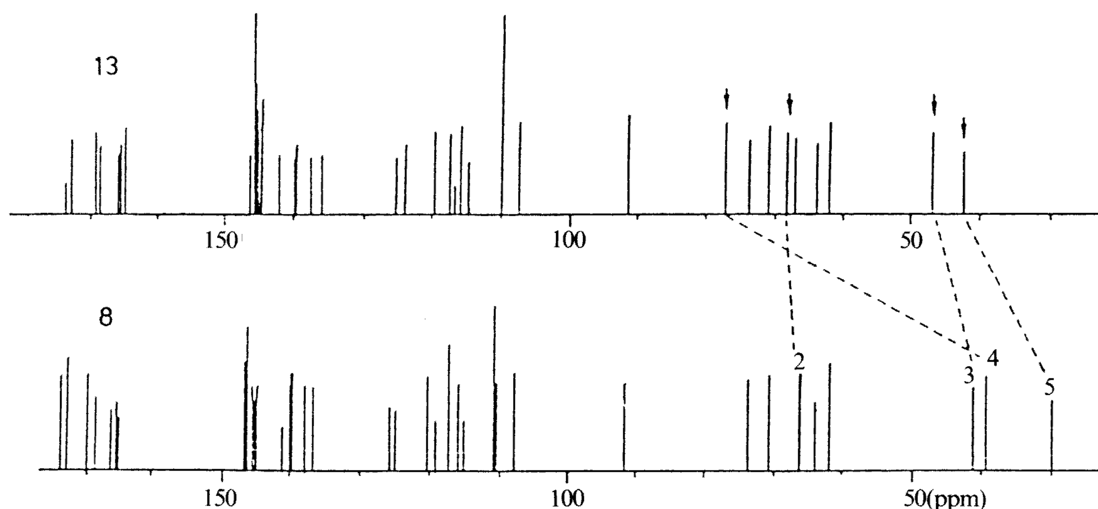
Figure 7. ^{13}\text{C-NMR} Spectra of Compounds 13 and 8 (in acetone- \text{d}_6 )
