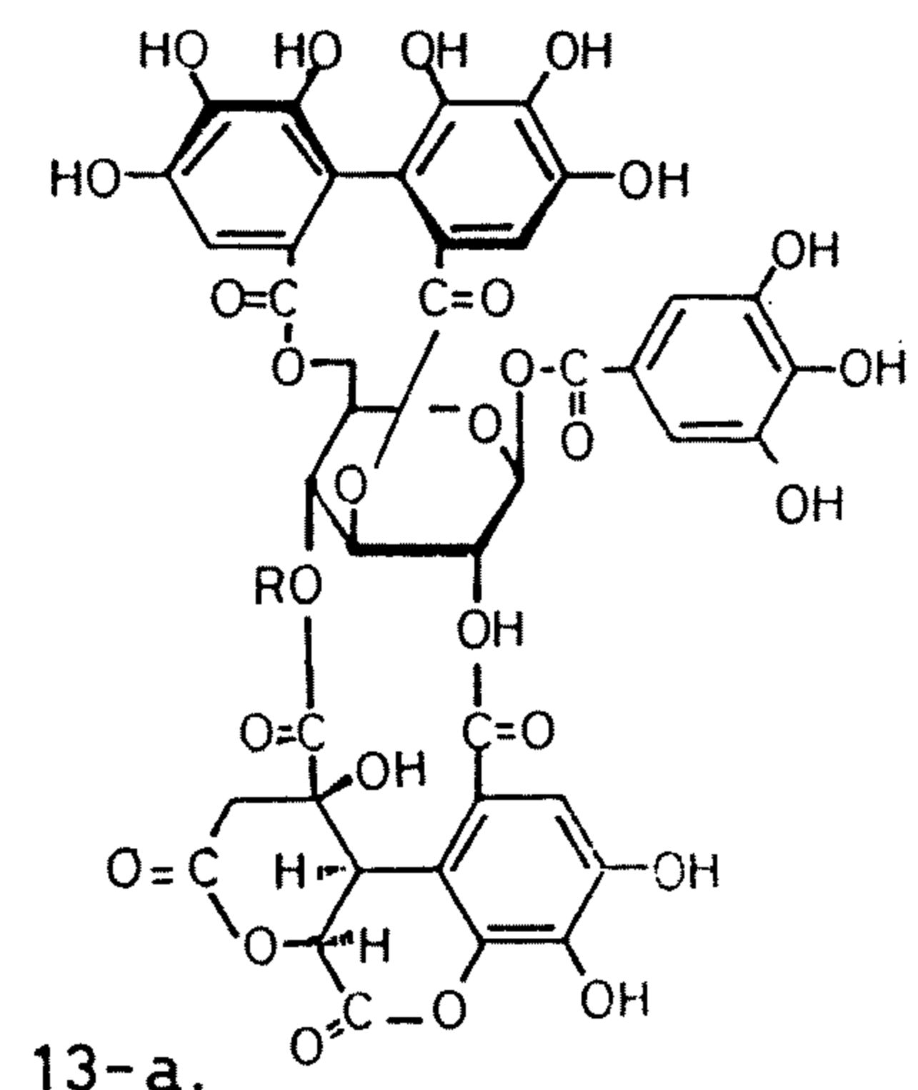
Figure 8. Structures of Compounds 13 and 13-a
