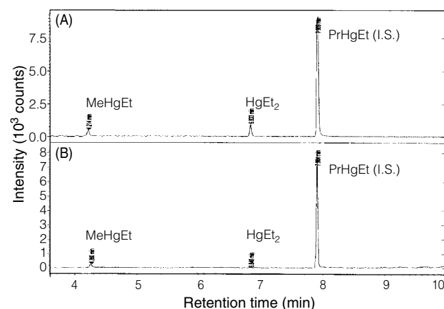
Figure 6. Gas chromatogram of (A) standard solution (1.0 \mu\text{g/mL} as Hg of methyl- and inorganic mercury and 2.0 \mu\text{g/mL} as Hg of propylmercury) and (B) laboratory tuna fish sample (1.98 \mu\text{g/g} methylmercury and 0.20 \mu\text{g/g} inorganic mercury). GC-ITMS conditions see Table 1.
