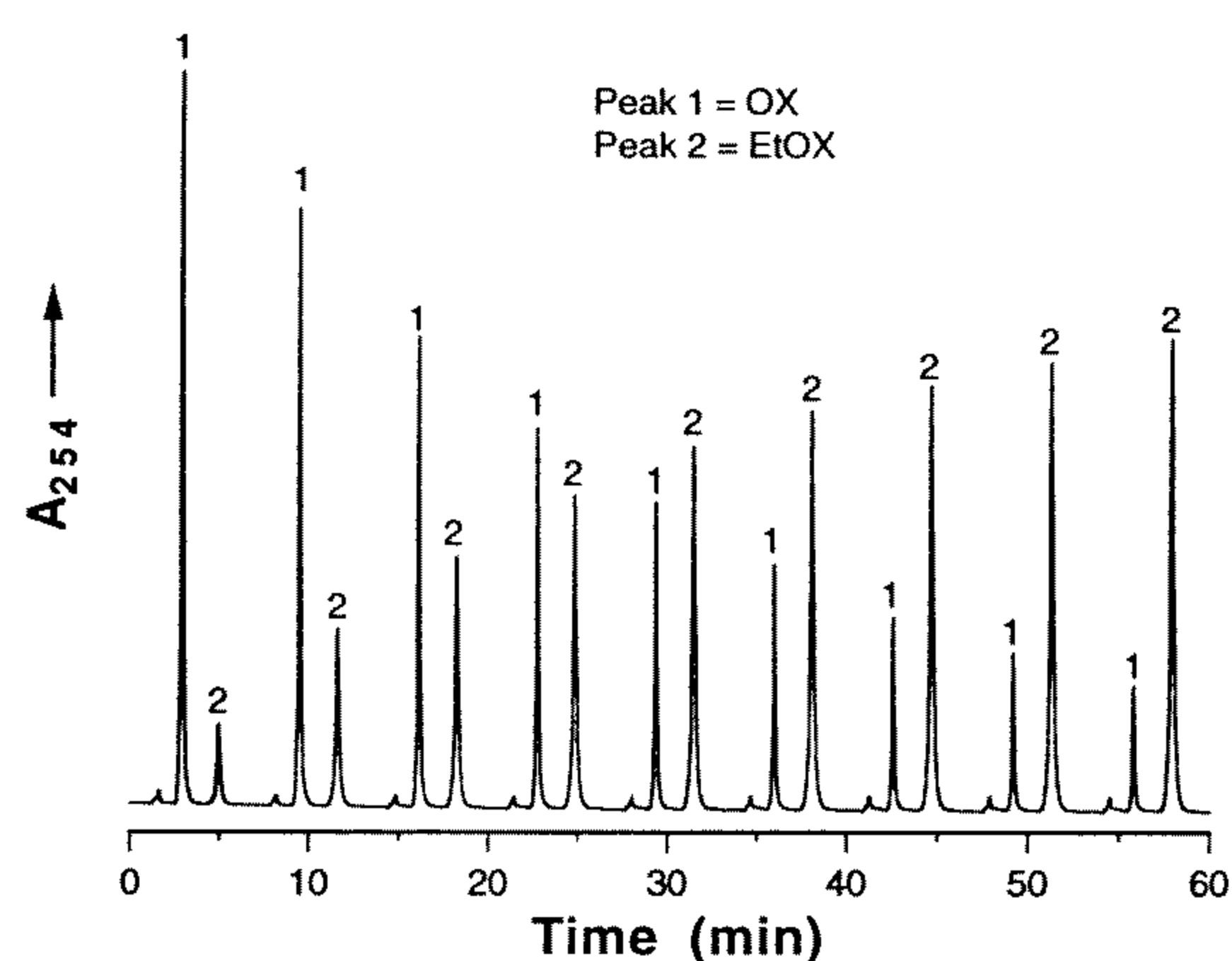
Fig. 2. Reversed-phase HPLC analysis in the continuous monitoring of acid-catalyzed ethanolysis of OX. Peaks 1 and 2 are OX and EtOX, respectively. OX (260 \mu g) in 1.5 ml of ethanol containing 0.1 M H_2SO_4 was maintained at 37°C. Aliquots (15 \mu l) were injected for analysis every 6.62 min. In the chromatogram shown, the t_{1/2} in the disappearance of OX was 21.5 min. HPLC conditions are described in Materials and Methods.
