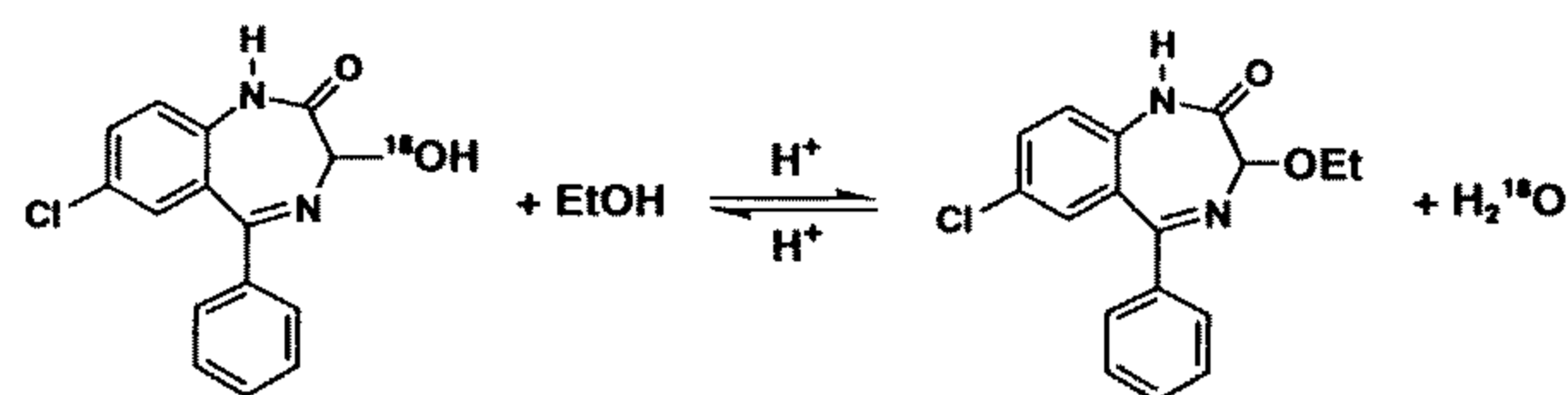
Fig. 4. Bond cleavages involved in acid-catalyzed ethanolysis of OX (forward reaction) and hydrolysis of EtOX (reverse reaction) as revealed by mass spectral analysis of product formations. See text for discussion.
