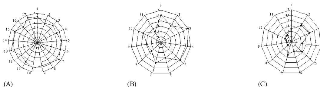
Figure 1. There are 17, 11 and 11 independent tests for genetically modified soybeans ( RRS ) for 5% (part A), 2% (part B) and 1% (part C) reference materials. Mean \pm SD values are 4.89 \pm 0.45 , 1.98 \pm 0.63 and 1.09 \pm 0.05 , respectively.
