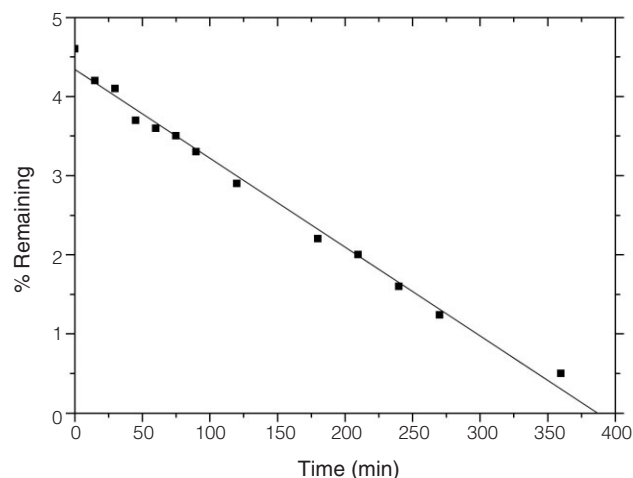
Figure 2. First-order plot for the degradation of compound 1b at pH 13.0 at 60°C
