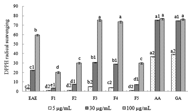
Figure 1 – DPPH radical scavenging activity of black garlic extracts and individual black garlic fractions (F1–F5).
