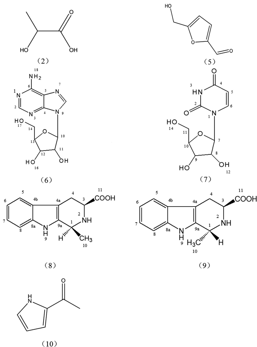
Figure 4 – Chemical structures of Compounds 2, 5, 6, 7, 8, 9, and 10 from black garlic: DL-lactic acid (2), 5-hydroxymethyl-2-furfural (5), adenosine (6), uridine (7), (1S,3S)-1-methyl-1,2,3,4-tetrahydro-β-carboline-3-carboxylic acid (8), (1R, 3S)-1-methyl-1,2,3,4-tetrahydro-β-carboline-3-carboxylic acid (9), and 2-acetylpyrrole (10).
