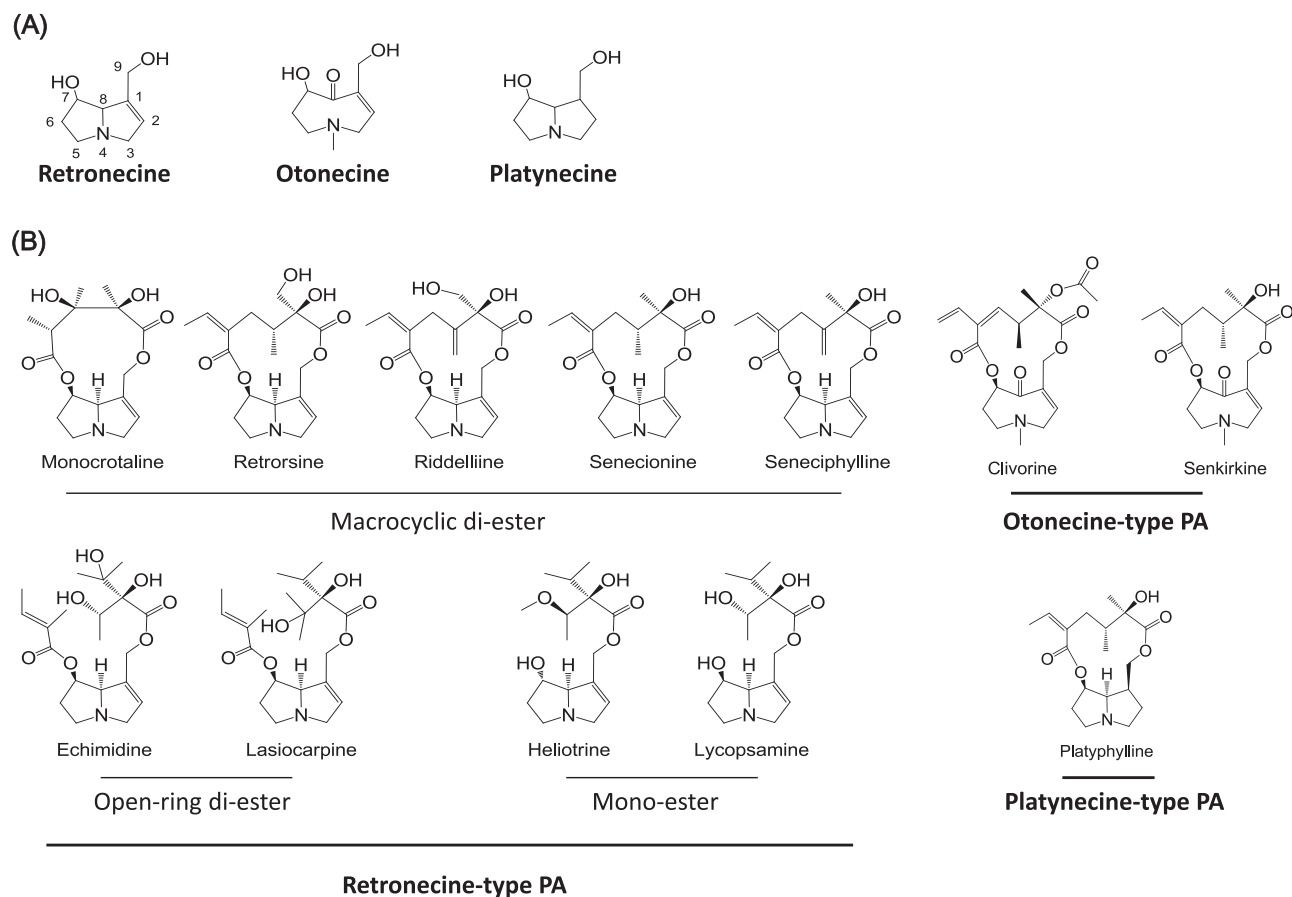
Fig. 1 – Chemical structures of the necine bases (A) and the representative PAs (B). Retronecine-type PAs can be further divided into three subgroups: macrocylic di-ester, open-ring di-ester, and mono-ester.
