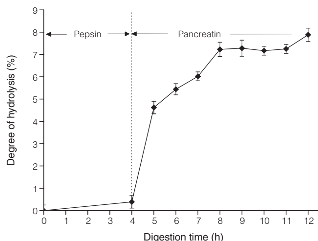
Figure 1. DH changes during simulated gastrointestinal digestion of AEVA. Data are presented as means \pm SD ( n = 3 ).
