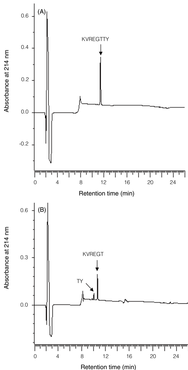
Figure 1. Stability of KVREGTTY during the incubation with ACE. RP-HPLC analysis of reaction mixtures before and after incubation with ACE on a LiChroCART C18 column (4 mm I.D. \times 250 mm). Chromatograms (A) before preincubation and (B) after preincubation with ACE. Peptide (0.02 mM) was incubated with 28 mU ACE (37°C, 3 hr).
