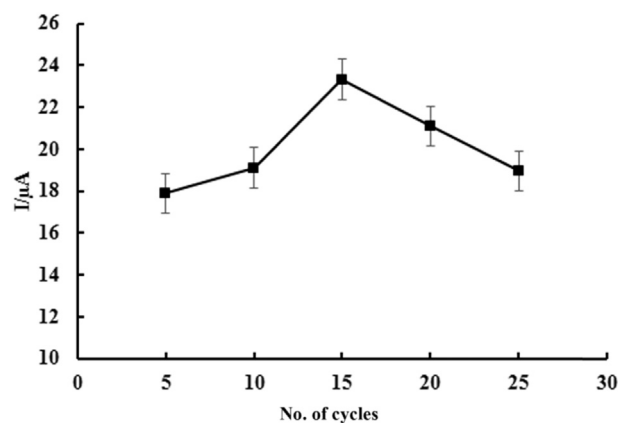
Figure 6 – Curve of peak current versus number of polymerization cycles. Supporting electrolyte is phosphate buffer solution of pH 3.0. Potential scan rate is 100 \text{ mV/s} .
