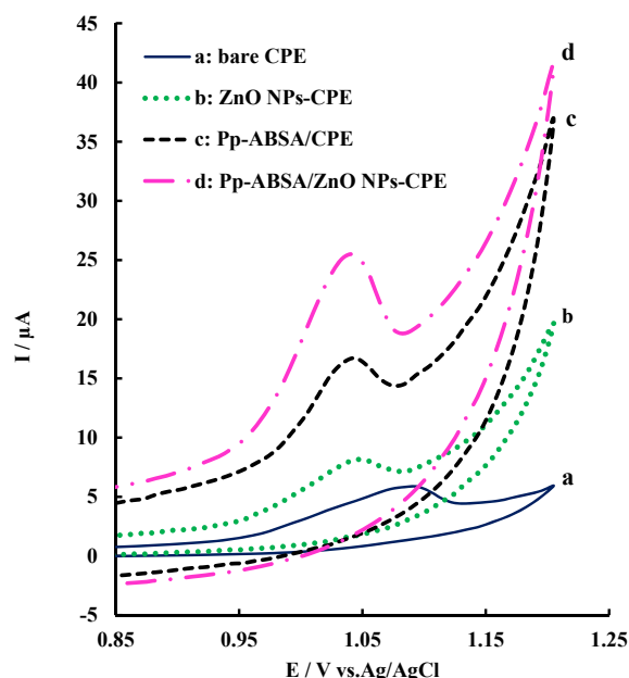
Figure 3 – Cyclic voltammogram responses ( I - E ) in phosphate buffer solution (PBS; 0.1 M, pH 3.0) and 5.98 \mu\text{M} tartrazine on (a) unmodified CPE, (b) ZnO NPs-CPE, (c) Pp-ABSA/CPE, and (d) Pp-ABSA/ZnO NPs-CPE. Scan rate = 100 \text{ mV/s} . CPE = carbon paste electrode; Pp-ABSA/CPE = poly ( p -aminobenzenesulfonic acid)/carbon paste electrode; Pp-ABSA/ZnO NPs-CPE = poly ( p -aminobenzenesulfonic acid)/zinc oxide nanoparticles carbon paste electrode; ZnO NPs-CPE = zinc oxide nanoparticles carbon paste electrode.
