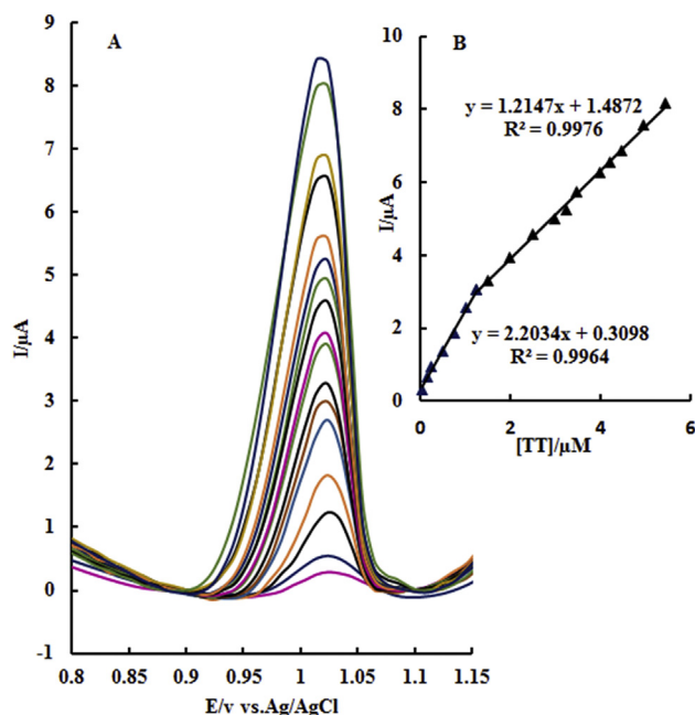
Figure 9 – (A) The differential pulse voltammogram responses of 0.1 M phosphate buffer solution (pH 3.0) with increasing tartrazine concentration on the poly ( p -aminobenzenesulfonic acid)/zinc oxide nanoparticles carbon paste electrode (Pp-ABSA/ZnO NPs-CPE); (B) the concentration calibration curve for tartrazine (TT).
