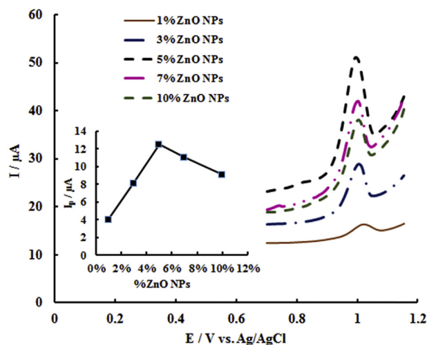
Figure 5 – Differential pulse voltammograms of 5.9 \mu\text{M} tartrazine on the surface of modified electrode with various amounts of zinc oxide nanoparticles (ZnO NPs); (inset) corresponding curve of peak current versus amount of ZnO NPs.
