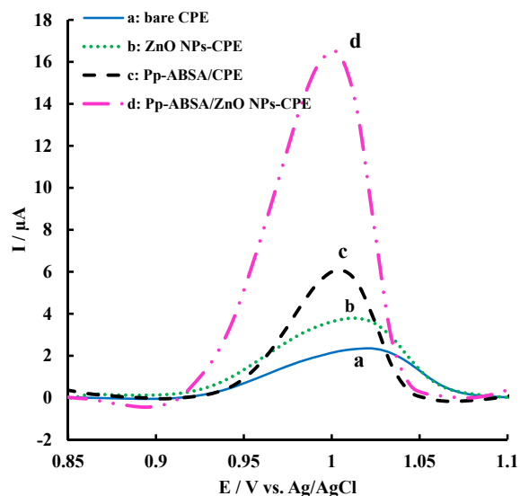
Figure 4 – Differential pulse voltammogram curves ( I - E ) of 1.49 \mu\text{M} tartrazine on (a) unmodified CPE, (b) ZnO NPs-CPE, (c) Pp-ABSA/CPE, and (d) Pp-ABSA/ZnO NPs-CPE. Scan rate = 20 \text{ mV/s} . CPE = carbon paste electrode; Pp-ABSA/CPE = poly ( p -aminobenzenesulfonic acid)/carbon paste electrode; Pp-ABSA/ZnO NPs-CPE = poly ( p -aminobenzenesulfonic acid)/zinc oxide nanoparticles carbon paste electrode; ZnO NPs-CPE = zinc oxide nanoparticles carbon paste electrode.
