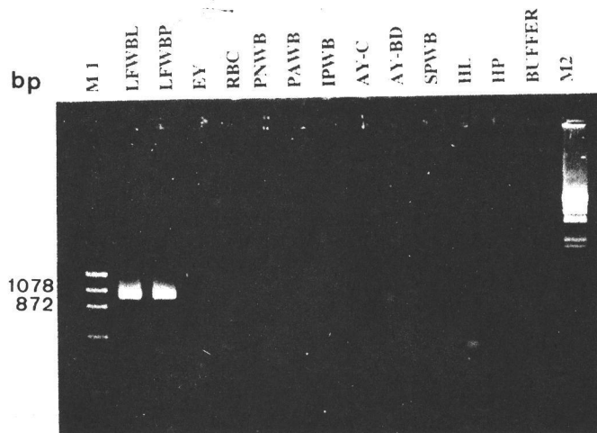
Fig. 2 Polymerase chain reaction (PCR)-analysis of DNA extracted from healthy plants and plants infected with mycoplasma-like organisms (MLOs). Reaction products are the results of PCR amplification with primer pairs p97F1-p97R1. DNA analysed by 1.5% agarose gel electrophoresis after staining with ethidium bromide, and the bands were visualized with ultraviolet light. Each strain description is the same as those in Table 1. Lane M1, molecular weight standards (in base pairs): 1353, 1078, 872, 603, 310, 281 + 271 bp from top band to bottom band. Lane M2, lambda DNA Hind III and EcoRI fragments
