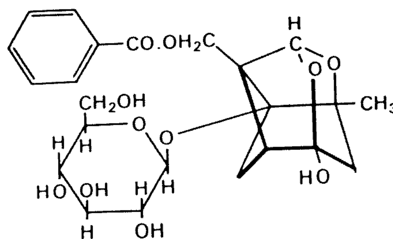
Figure 1. Structure of paeoniflorin
