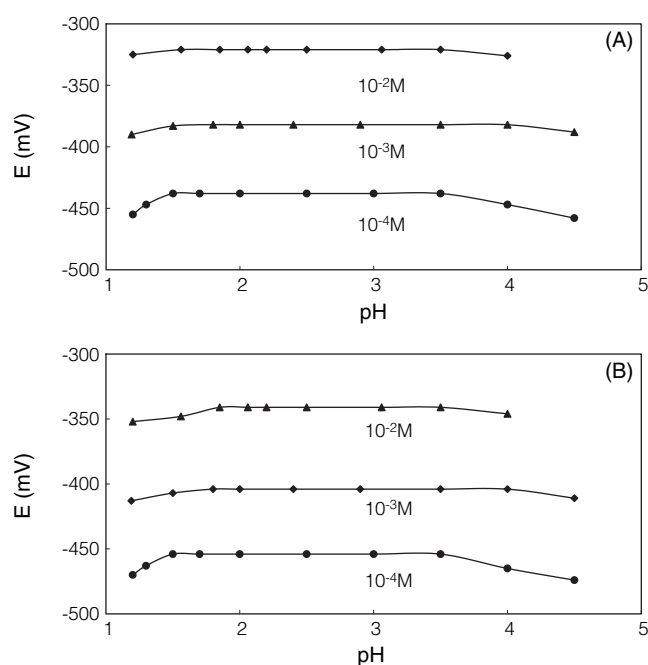
Figure 4. pH – potential profile of TpCIPB-clopidogrel PVC based membrane sensor. (A) DOP and (B) o -NPOE.
