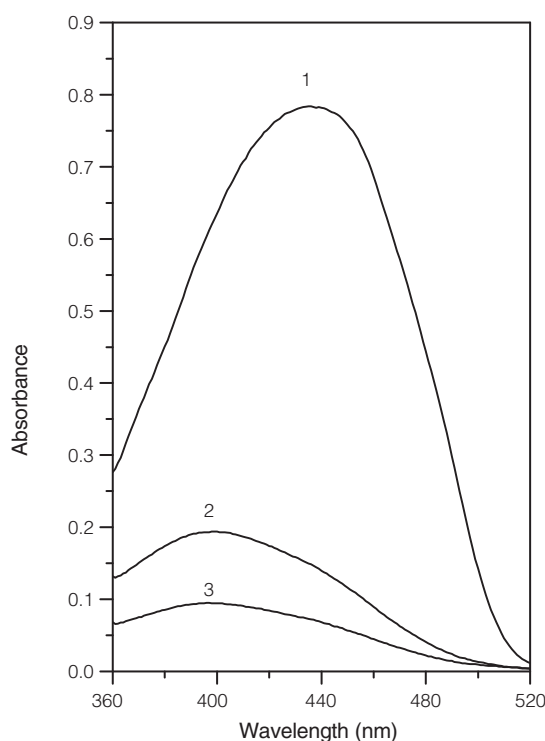
Figure 2. Absorption spectra of tartrazine in solution and \beta -CDP solid-phase. 1, Tartrazine in \beta -CDP solid-phase; 2, tartrazine in solution in the presence of \beta -CD; 3, tartrazine in solution in the absence of \beta -CD. The condition is pH=1, \beta -CDP (60–80 mesh): 0.5 g, tartrazine (200 µg/mL) 1 mL, shaking time: 40 min, room temperature, total volume: 25 mL.
