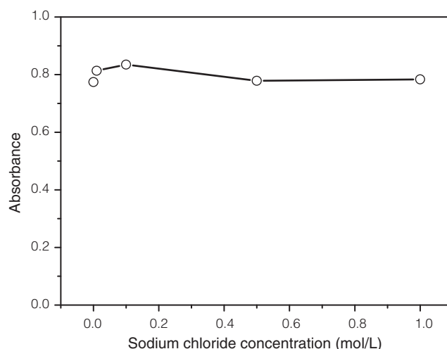
Figure 6. Effect of ionic strength on \beta -CDP including tartrazine. The condition is pH=1, \beta -CDP (60-80 mesh): 0.5 g, tartrazine (200 \mu\text{g/mL} ): 1 mL, shaking time: 40 min, room temperature, total volume: 25 mL.
