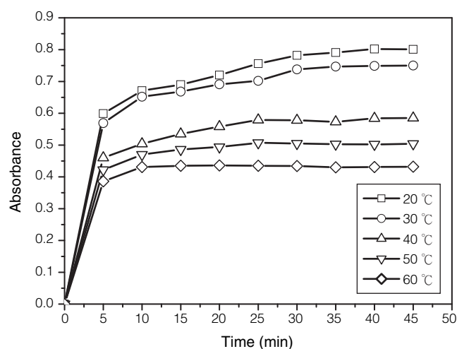
Figure 4. Effect of temperature and time on \beta -CDP including tartrazine. The condition is pH=1, \beta -CDP (60-80 mesh): 0.5 g, tartrazine (200 \mu g/mL): 1 mL, total volume: 25 mL.
