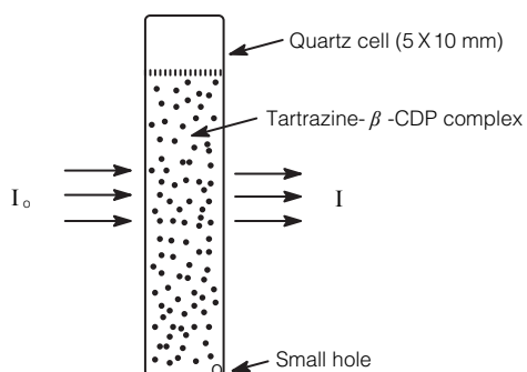
Figure 1. The quartz cell used and packing manner of tartrazine- \beta -CDP complex.
