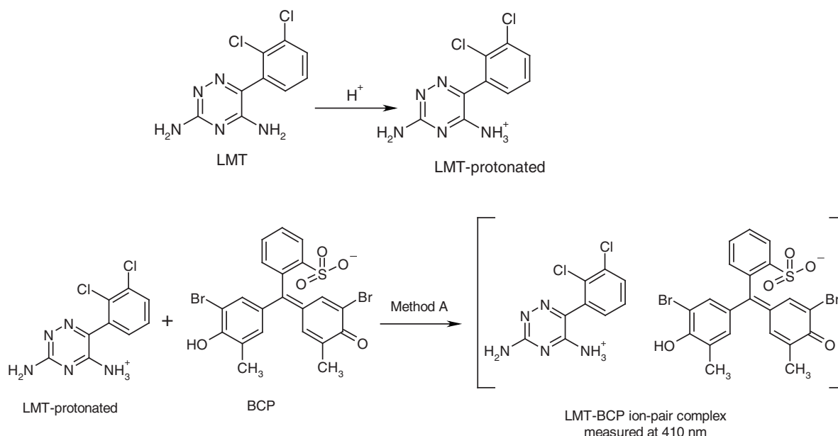
Scheme 1. Proposal of the reaction pathway to form ion-pair complex between the drug and dye.
