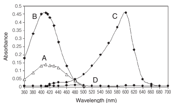
Figure 1. Absorption spectra of ion-pair complex and various forms of dye. A: ion-pair complex (4.0 \mu\text{g/mL} LMT); B: acid form of dye (750 ng/mL LMT); C: base form of dye (275 ng/mL LMT) and D: blank.
