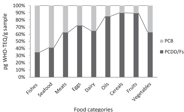
Figure 1 – Levels of polychlorinated dibenzo-p-dioxin/polychlorinated dibenzofuran (PCDD/Fs) and polychlorinated biphenyl (PCBs) in alternative food categories. TEQ = toxic equivalency factor; WHO = World Health Organization.
