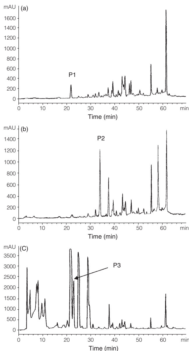
Figure 2. Fingerprint chromatograms of (a) Euphorbia ebracteolata Hayata, (b) Euphorbia fischeriana Steud, and (c) Stellera chamaejasme L. (Note: P1 = Ebracteolata compound B, P2 = Jolkinolide B and P3 = Neochanmaejasmin)
