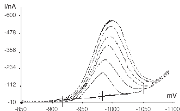
Figure 2. Adsorptive stripping voltammogram for enoxacin indicating potential (mV) versus current (nA) in 0.1 M HCl, pH 1.8, peak potential 0.98 V, concentrations 1–30 \mu\text{g}/\text{mL}^{-1} enoxacin.
