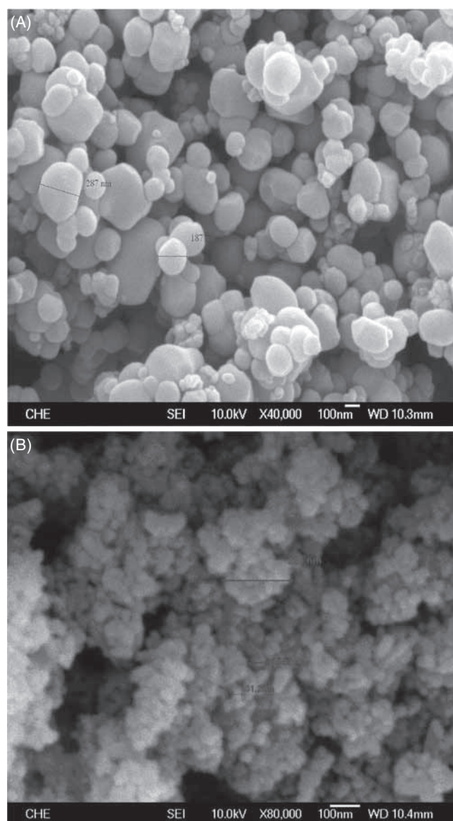
Figure 3. (A) SEM of submicron-sized \text{TiO}_2 in glycerin dispersion. (B) SEM of nanosized \text{TiO}_2 in glycerin dispersion.
