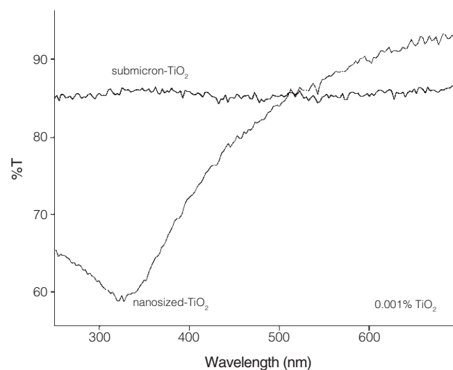
Figure 2. UV-visible transmittance spectra of submicron-sized \text{TiO}_2 and nanosized \text{TiO}_2 at 0.001% concentration in water.
