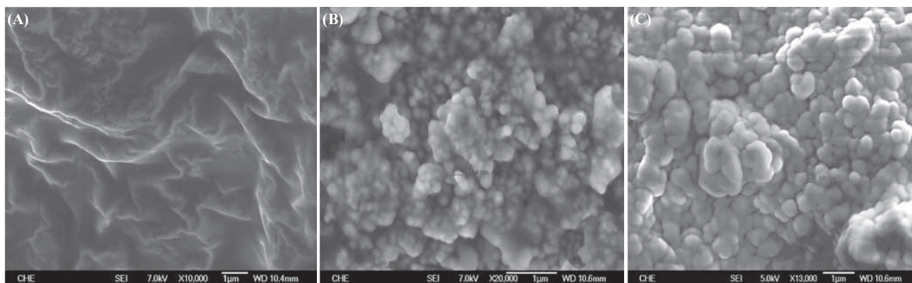
Figure 7. (A) SEM of cream base. (B) SEM of cream containing 20% submicron-sized \text{TiO}_2 . (C) SEM of cream containing 20% nanosized \text{TiO}_2 .
