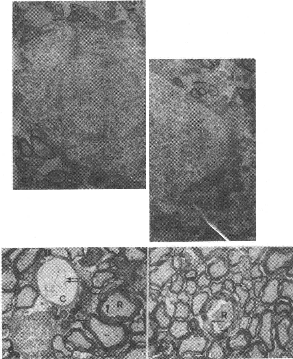
Fig. 6. Electron micrographs of the left AVCN (A-C) and right AVCN (D-I) at three months after right ligation. A few microcysts (arrows), probably derived from edematous dendrites, closely contact or are adjacent to a neuronal cell (A). A blood vessel (C) contains a membranous structure (double arrows) in its lumen and a vacuole (double arrowheads) in the endothelial cell (B). An adjacent pericyte contains several multivesicular bodies (single arrows). Note the detachment (single arrowhead) of the myelin sheath from the retracted axon (R). Disruption (arrow) and detachment (arrowhead) of the myelin sheath are found in the right AVCN (C). Disruption of the myelin sheath (arrow) is found in the right AVCN (D). Vacuoles (arrows) are found in the cytoplasm near the peripheral plasmalemma in the ipsilateral AVCN (E). The myelin sheath (arrows) protrudes into the myelinated nerve fiber in the ipsilateral AVCN (F). Vacuoles (arrows) are closely contacting the nuclei (N) (G) or are found in the cytoplasm near the peripheral plasmalemma (H) of the superficial granule cell in the right AVCN. Note the detachment (arrowhead) of the myelin sheath (G). Edematous dendrites (arrows) corresponding to the foamy region are found in the neighboring cells (I). Large vacuoles are frequently found in edematous dendrites (arrows) or are closely associated with the disruption of the myelin sheath (double arrowheads). Scale bar: 2 \mu m.
