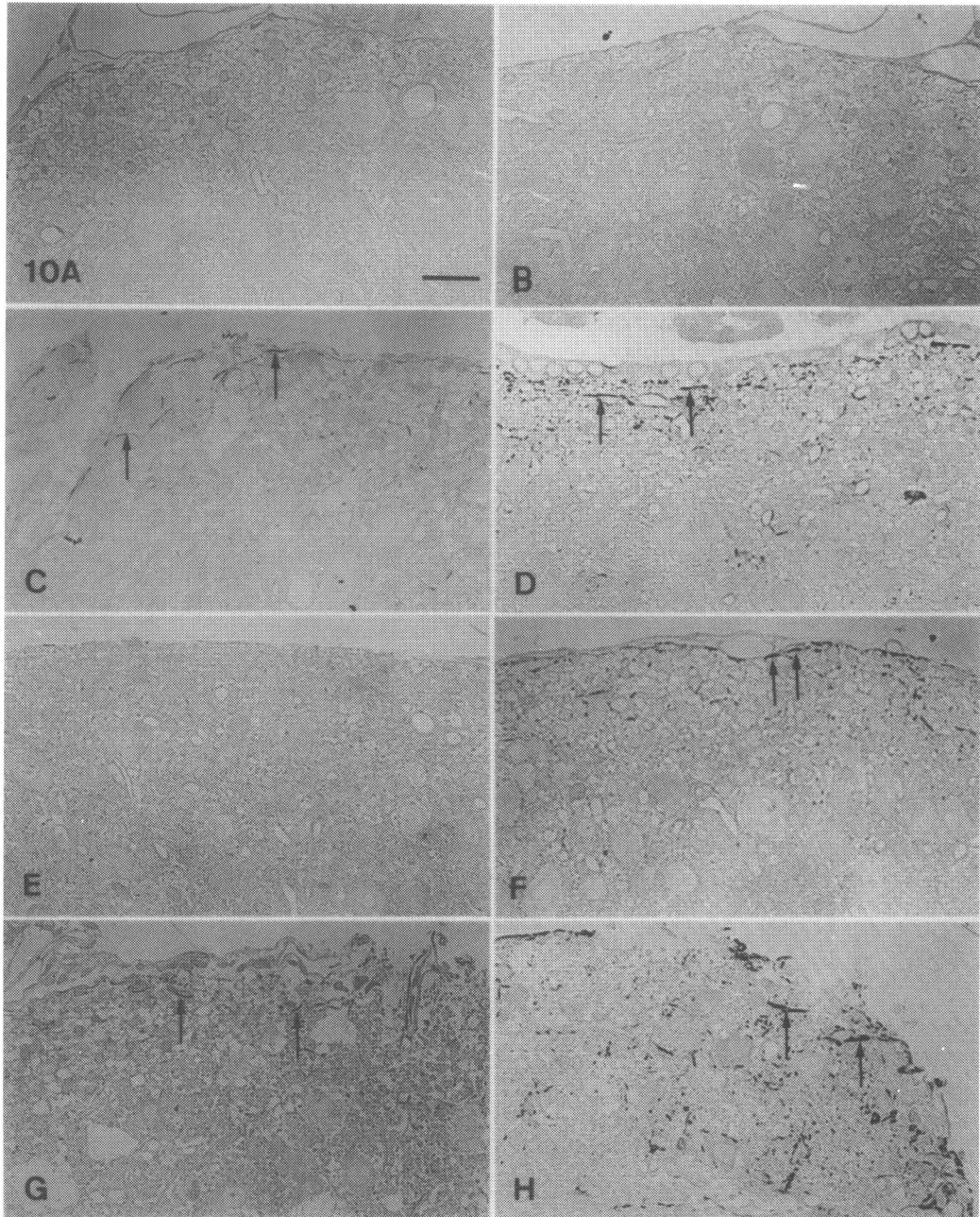
Fig. 10. Light micrographs of GFAP-IR in the superficial layer of the left (A, C, E, G) and right (B, D, F, H) AVCN. GFAP-IR is not immunolabeled in the left (A) and right (B) AVCN at one month after right ligation. GFAP-IR is immunolabeled in the left (C) and right (D) AVCN. GFAP-IR is immunolabeled more intensely in the right AVCN (D) than in the left (C). At six months after right ligation, GFAP-IR is not immunolabeled in the left AVCN (E) but is slightly reduced in the right (F). At nine months after right ligation, GFAP-IR is immunolabeled in the left AVCN (G) and in the right (H). GFAP-IR is immunolabeled more intensely in the right AVCN (H) than in the left (G). Scale bar: 25 \mu m.
