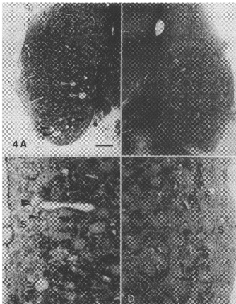
Fig. 4. Light micrographs of the left AVCN (A,B) and right AVCN (C,D) at nine months after right ligation. Numerous microcysts (arrows) remained in the left AVCN (A). Some of the microcysts (double arrowheads) are found at the junction of the superficial granule cell cap and the deep layer, and the vacuoles (arrows) in the neuronal cells of the left AVCN (B). Note that the vacuole (single arrowhead) contains vesicles. A foamy region is more evident in the superficial granule cell cap (S) of the left AVCN (B) than in that of the right AVCN (D). No vacuoles are found in the right AVCN (D). Scale bar: 100 µm for A and C, and 25 µm for B and D.
