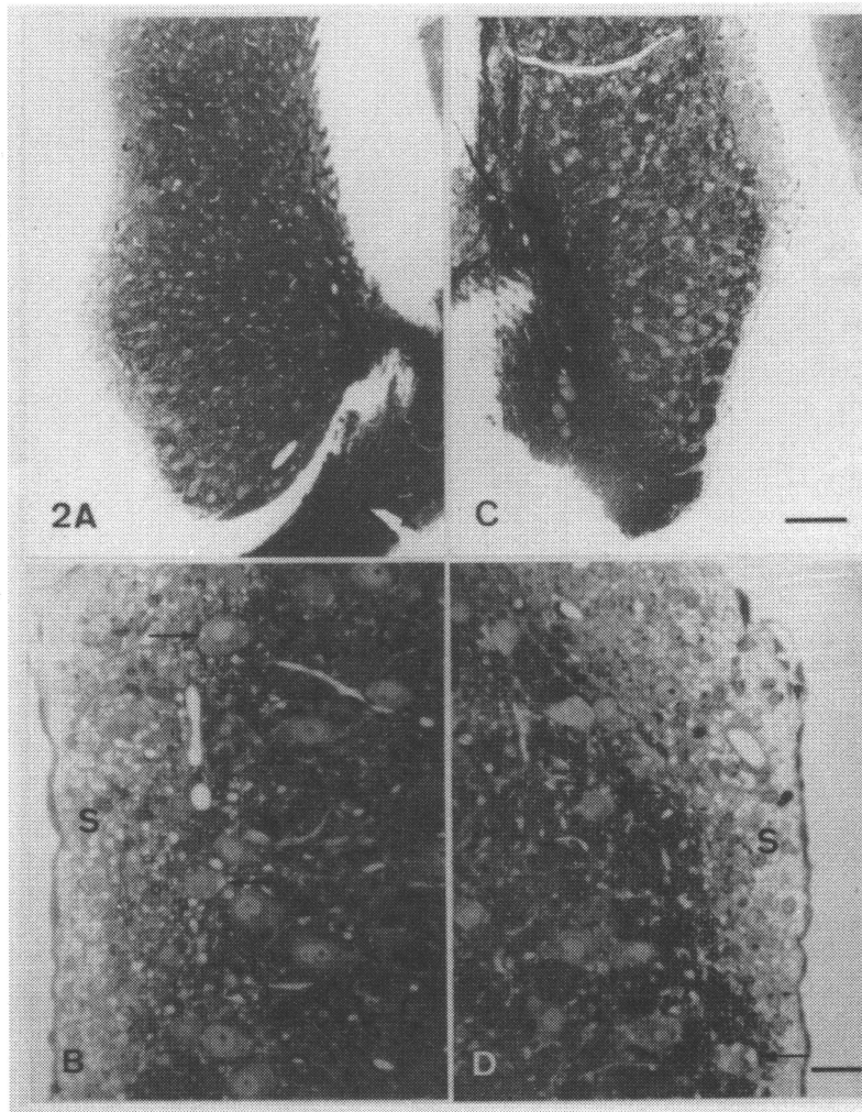
Fig. 2. Light micrographs of the left AVCN (A,B) and right AVCN (C,D) at three months after right ligation. No discernible microcysts are found in the AVCN (A,C). A foamy region becomes evident in the superficial granule cell cap (S) of the left (B) and right (D) AVCN. A few vacuoles are found in the neuronal cells (arrows) adjacent to the superficial granule cell cap (S) in the left (B) and right (D) AVCN. Scale bar: 100 µm for A and C, and 25 µm for B and D.
