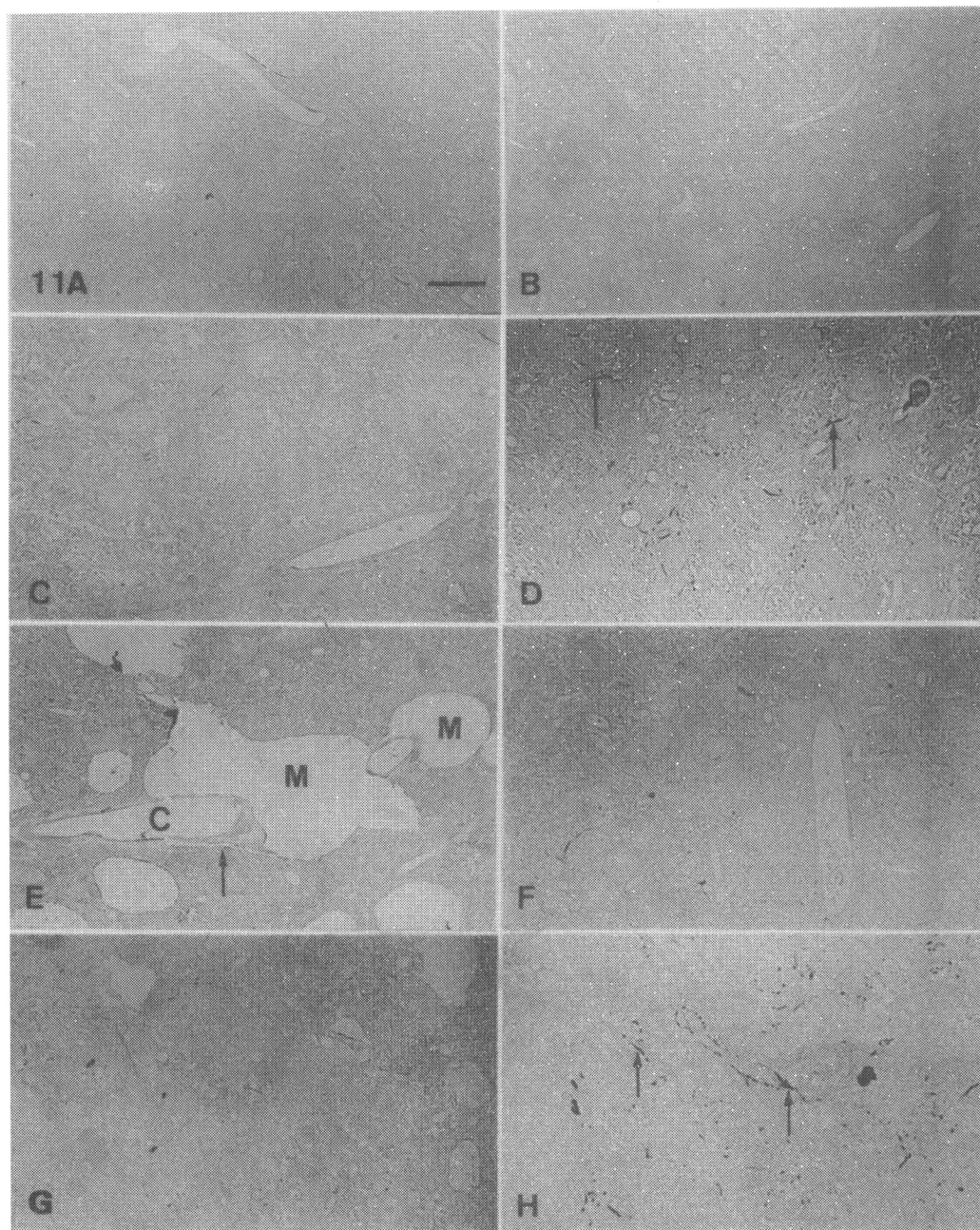
Fig. 11. Light micrographs of GFAP-IR in the deep layer of the left (A, C, E, G) and right (B, D, F, H) AVCN. No discernible GFAP-IR is immunolabeled in the left (A) or right (B) AVCN at one month after right ligation. At three months after right ligation, GFAP-IR is not immunolabeled in the left AVCN (C) but is immunolabeled in the right (D). At six months after right ligation, no discernible GFAP-IR is immunolabeled in the left (E) or right (F) AVCN. At nine months after right ligation, GFAP-IR is not immunolabeled in the left AVCN (G) but is immunolabeled in the right (H). Scale bar: 25 \mu m.
